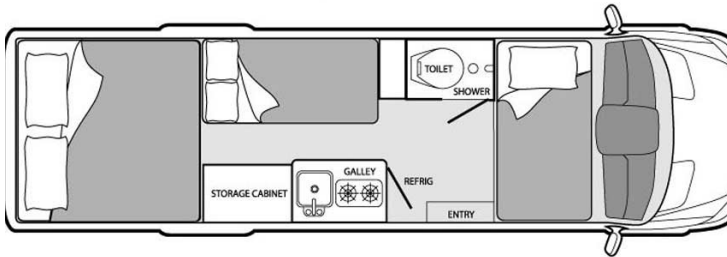
Clanhauler Campervan Floor Plan
