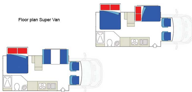
Floor plan Midi Motorhome Jour/Day
